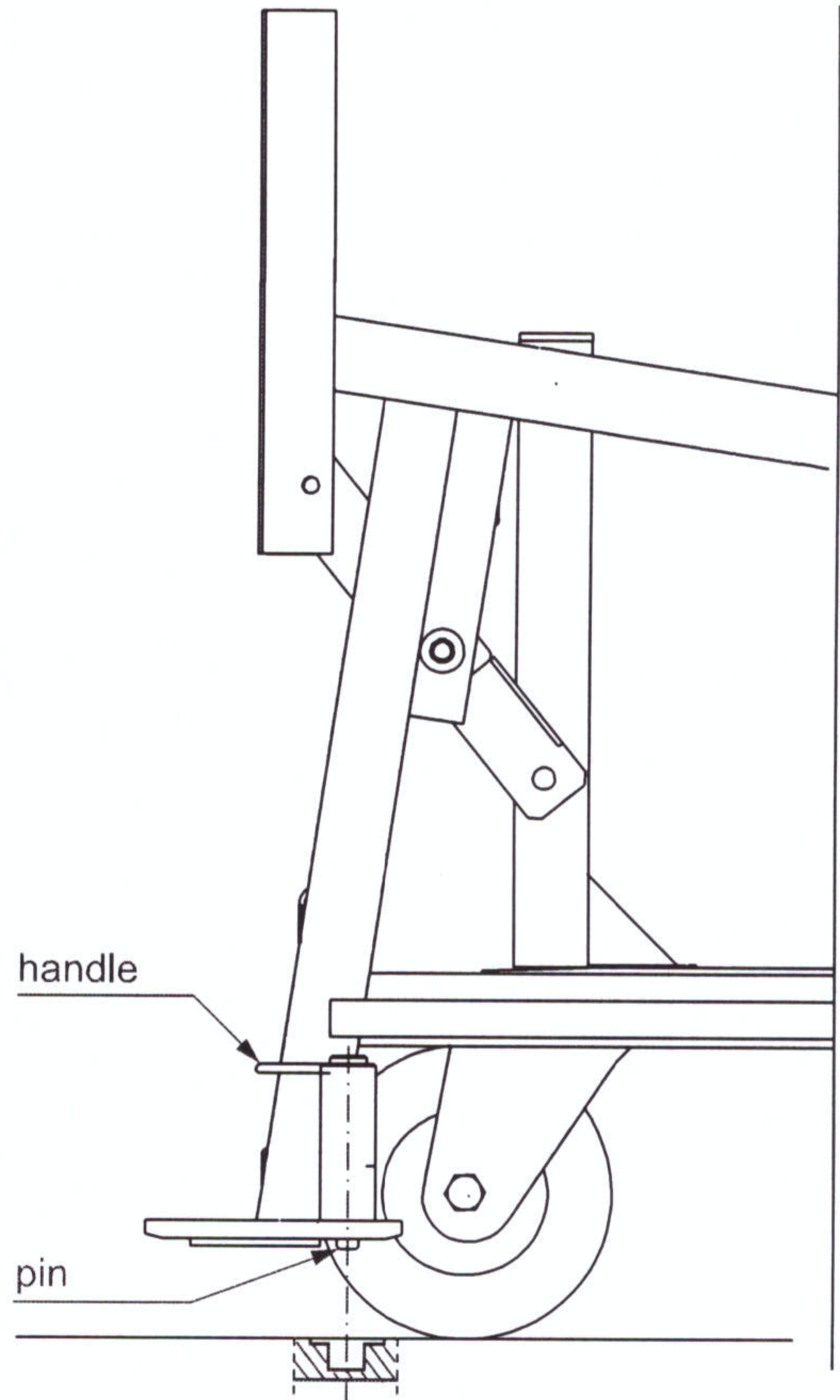
Pic.4 Sight of alignment pin and position of base footing - storing position
